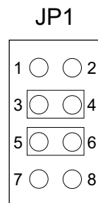
unipolar 0...10V
